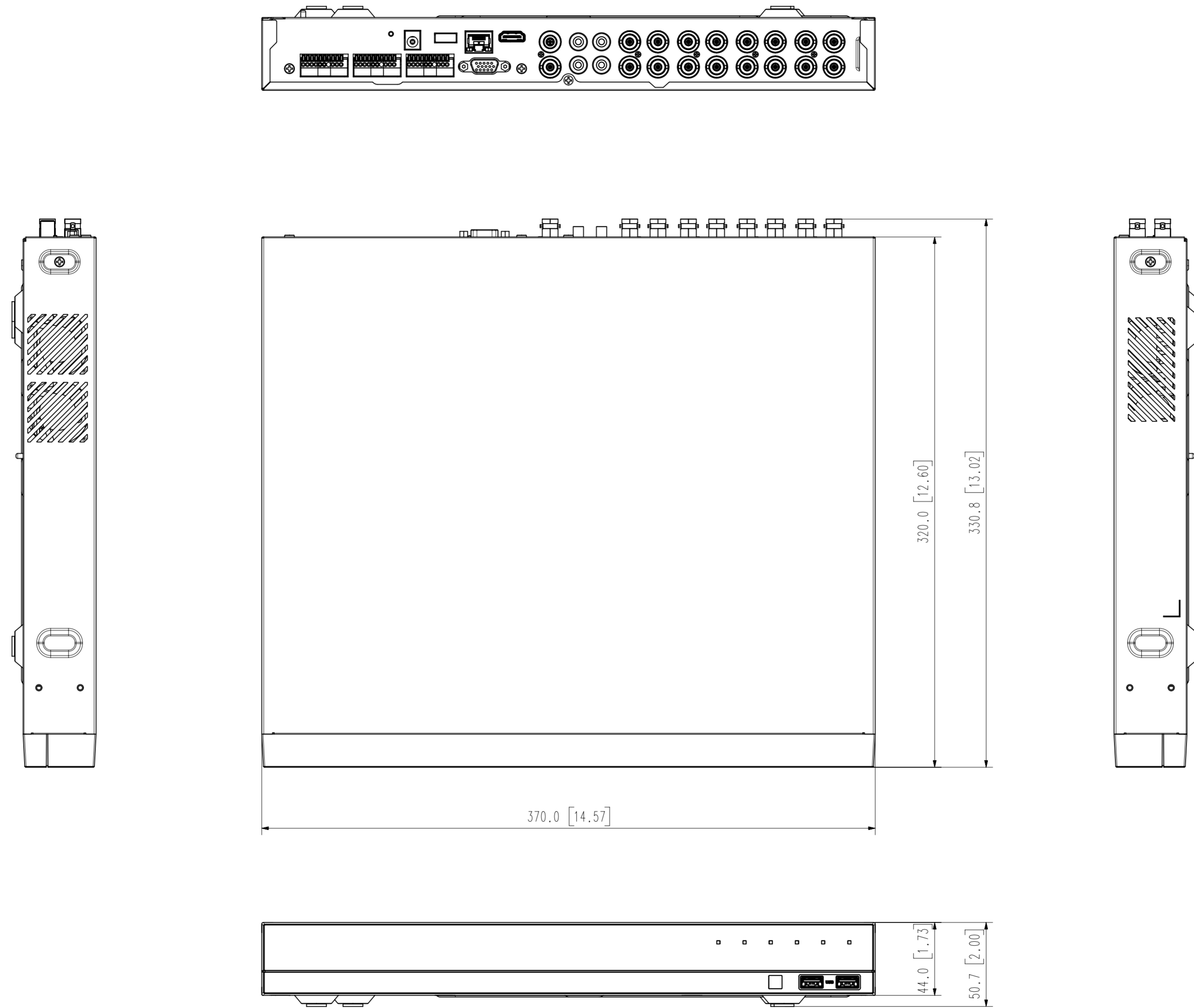
Appearance drawing HRX-1620 Unit : mm[inches]
