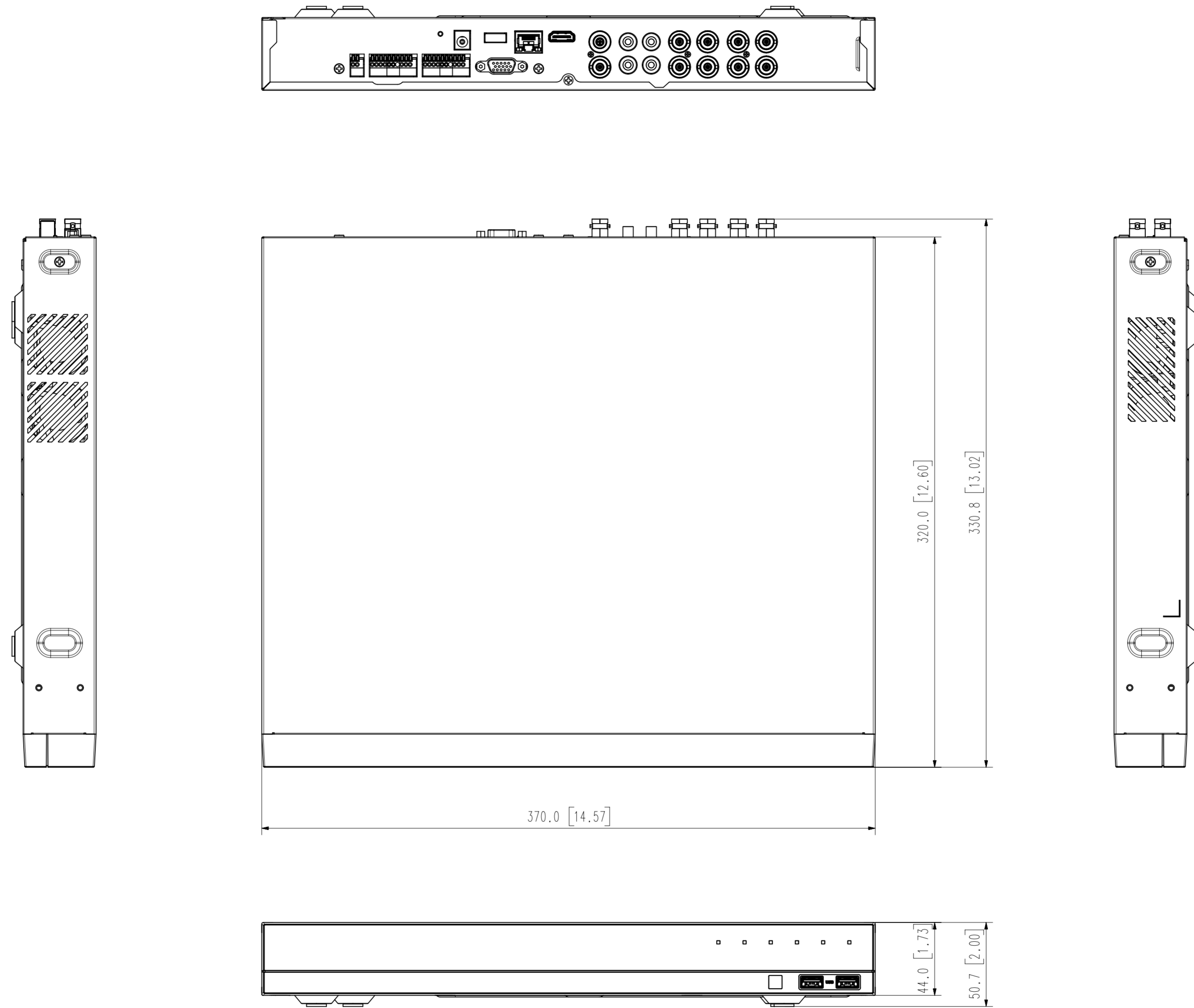
Appearance drawing HRX-820 Unit : mm[inches]
